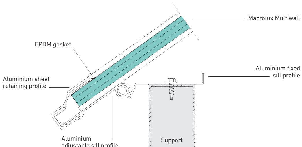
SCHEME [ C ] Lateral view
