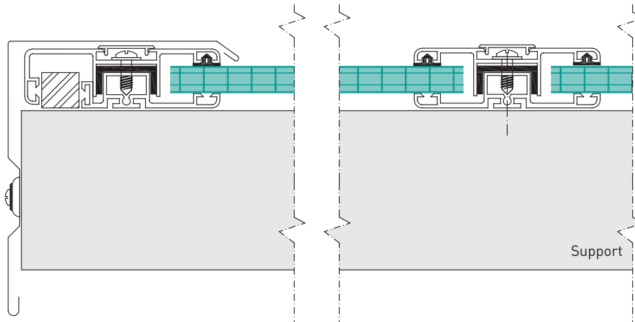
SCHEME [ A ] Aluminium head profile
